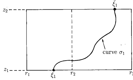
FIG. 10. Construction of the curve \sigma_1 in R_1 .
