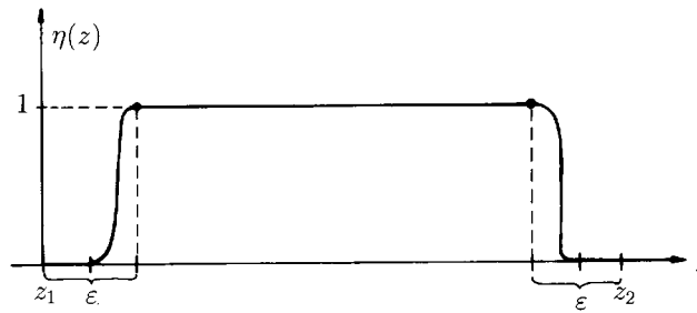
FIG. 12. Properties of the test function \eta .
